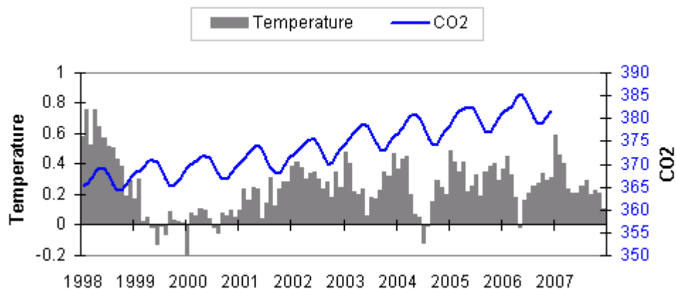
Figure 1-2. UAH lower tropospheric temperatures and carbon dioxide over last 10 years.
