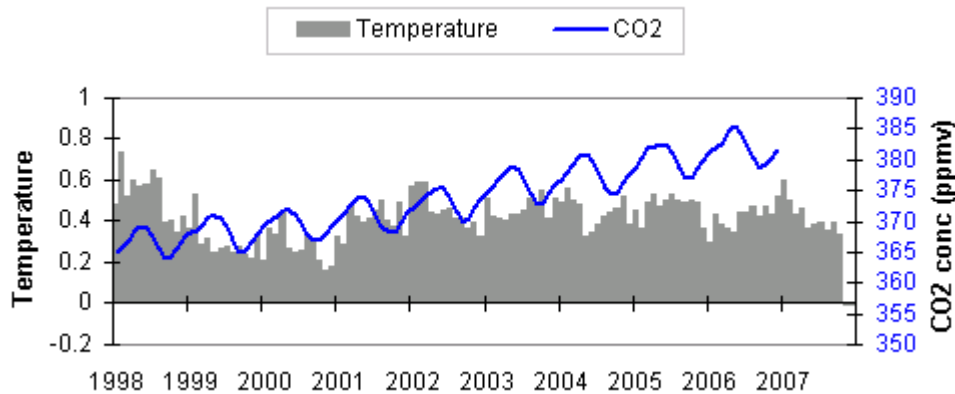
Figure 1-1. HadCRUT3v average global temperature and carbon dioxide over last 10 years
