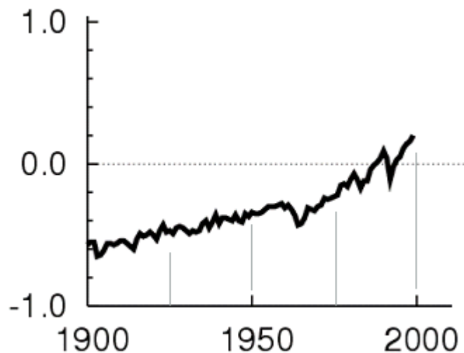
Figure 4-1. Estimated historical annual average temperature anomalies according to 23 climate models (part figure SPM-5 of IPCC WG I report)
