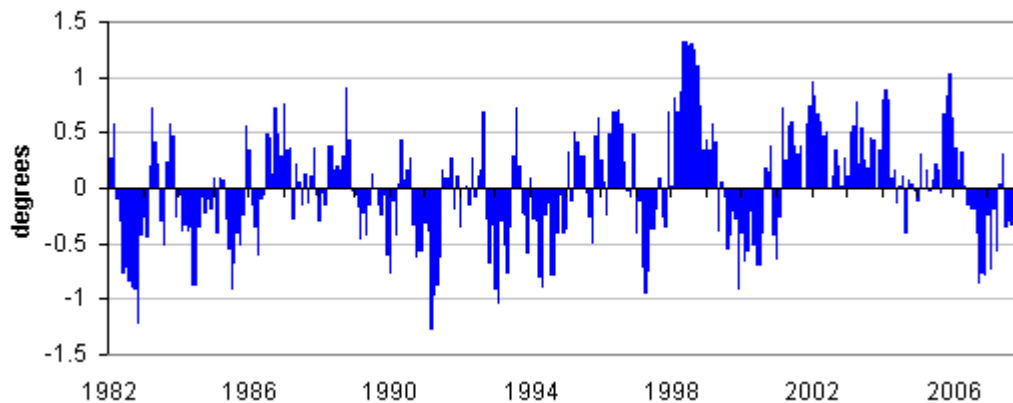
Figure 7-12. Sea surface temperature anomalies for the Great Barrier Reef
