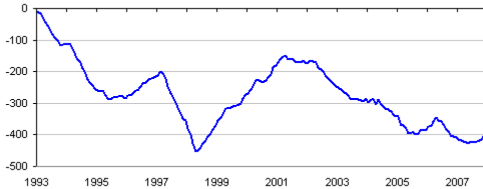
Figure 7-14. Aggregated monthly SOI over the same period as 7-13 illustrates the bias to negative SOI conditions (i.e. towards El Nino).
