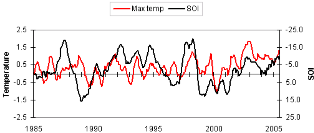
Figure 7-3d. Maximum temperature and SOI
