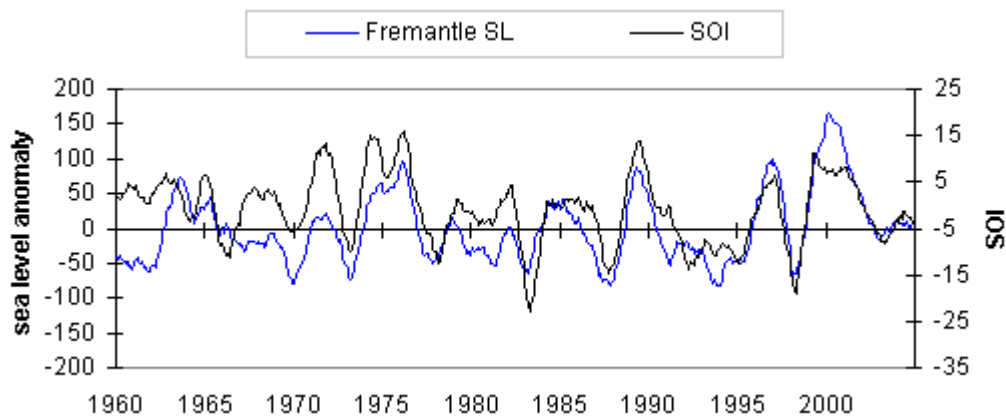
Figure 7-5. Sea level anomalies at Fremantle (WA) and SOI
