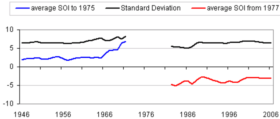
Figure 6-13. Average SOI to 1975 and from 1977, and standard deviation
