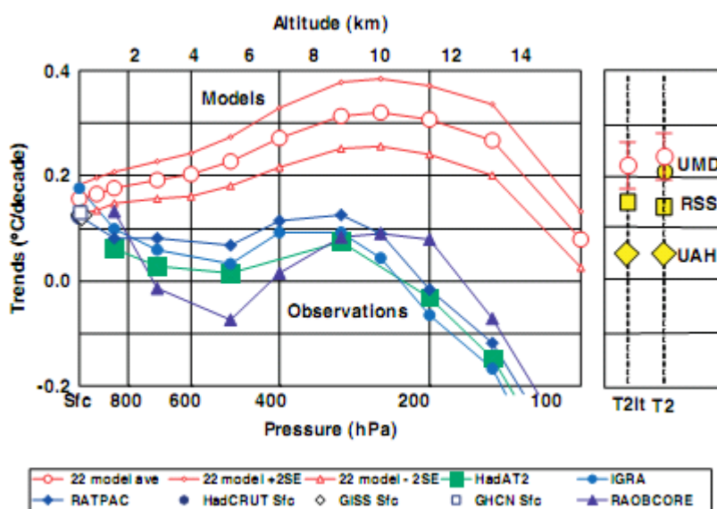
Figure 6-4. Predicted and observed trends for lower tropospheric temperatures
