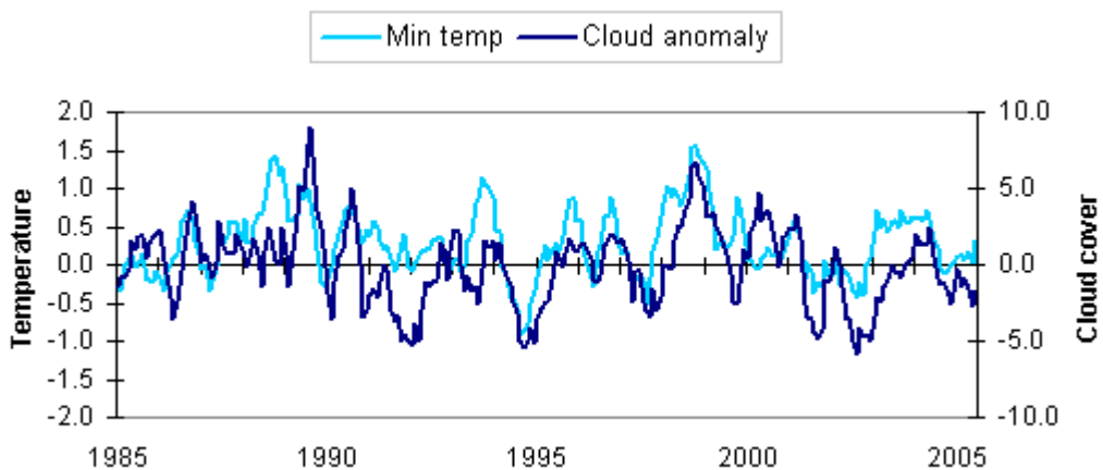
Figure 7-3c. Minimum temperature and cloud cover
