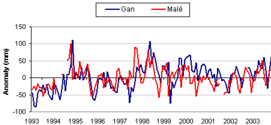
Figure 6-7: Monthly sea level anomaly for two locations in The Maldives
