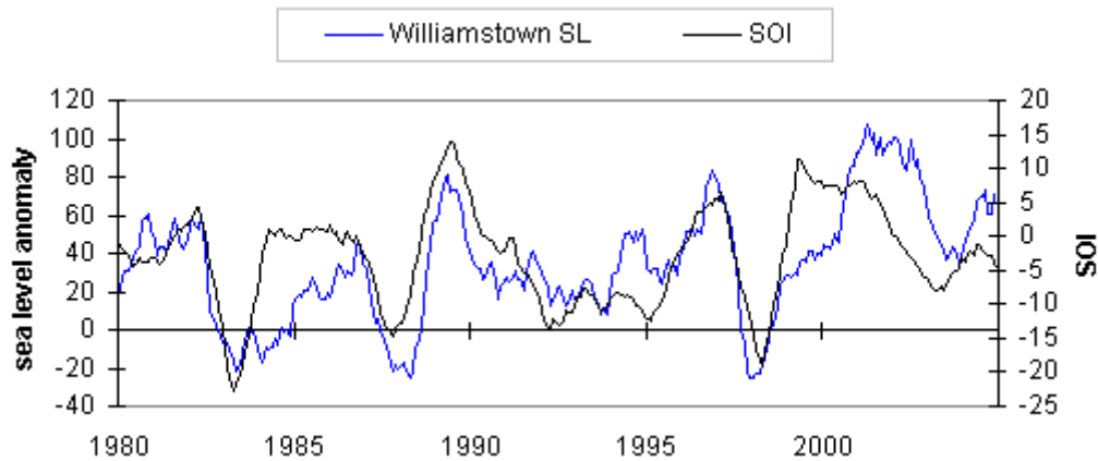
Figure 7.6. Sea level anomalies at Williamstown (Vic) and SOI
