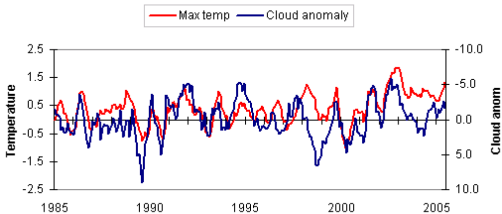
Figure 7-3b. Maximum temperature and inverted cloud cover
