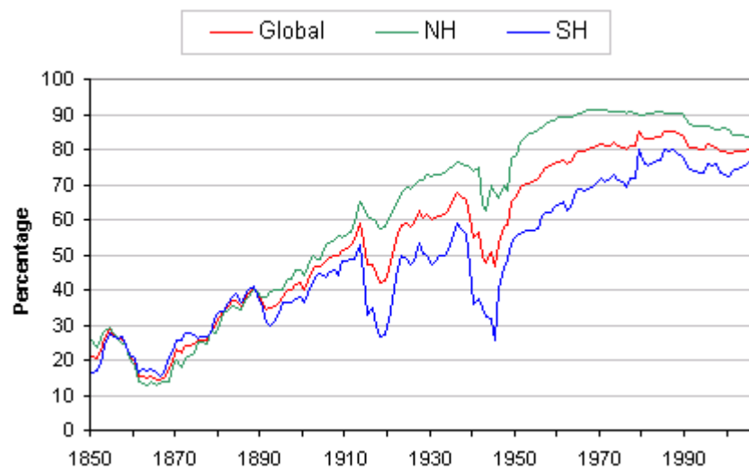
Figure 6-5. Coverage of the HadCRUT3v temperature data (hemispheric and global)
