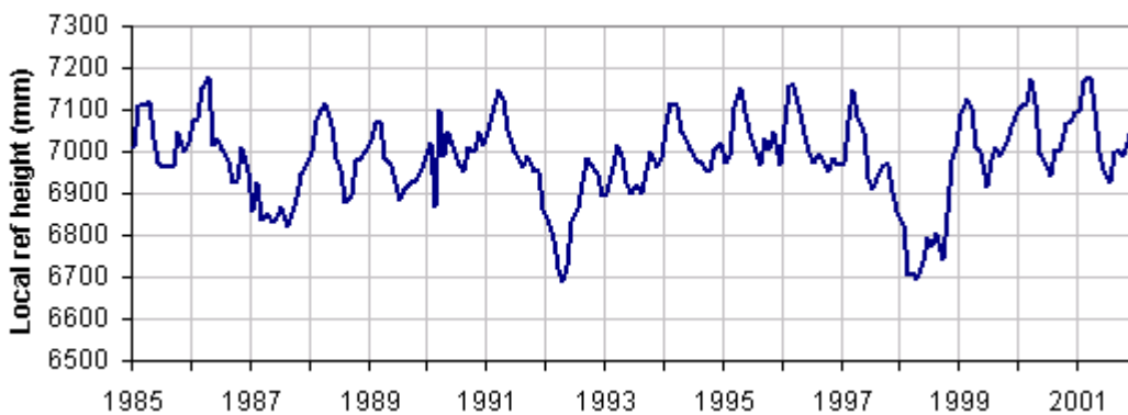
Figure 6-8: Sea level at Funafuti, located on one of the islands of Tuvalu.
