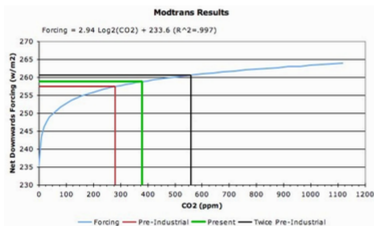
Figure 6-1. Downward radiation caused by carbon dioxide, according to MODTRAN software
