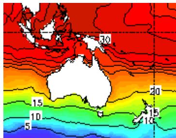
Figure 7-4 Sea surface temperatures around Australia in June 2001
