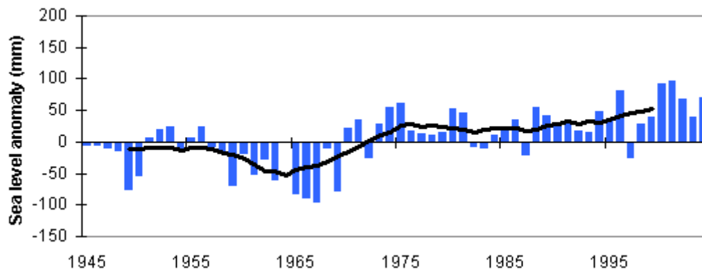
Figure 7-9 Annual average sea level anomaly and 11-year average at Williamstown. Changed to a new gauge, which was reporting sea level 88mm higher, in January 1970
