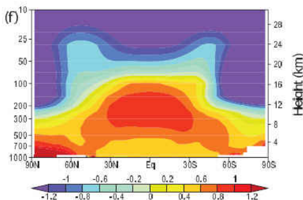
Figure 6-2a. Predicted temperatures trends in the lower troposphere according to the IPCC (period=1890-1999)
