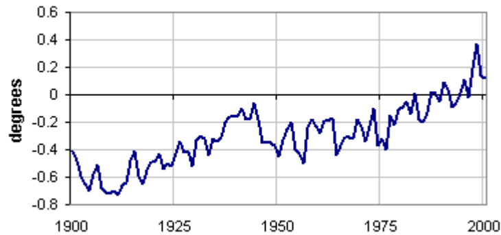
Figure 4-2. Annual average temperatures according to CRU data (0 line = average 1980-99)
