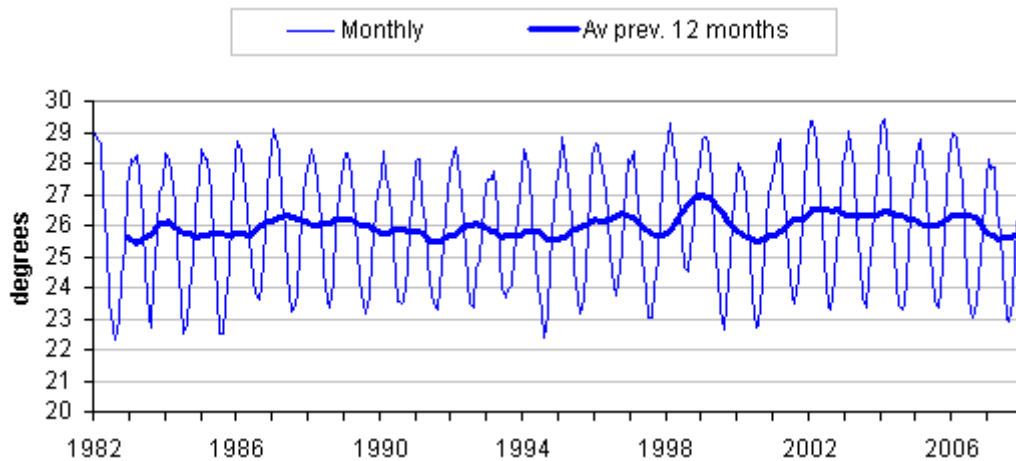
Figure 7-11. Sea surface temperatures across the Great Barrier Reef
