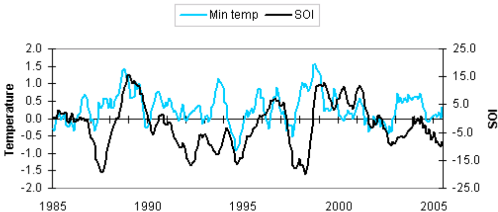
Figure 7-3e. Minimum temperature and SOI
