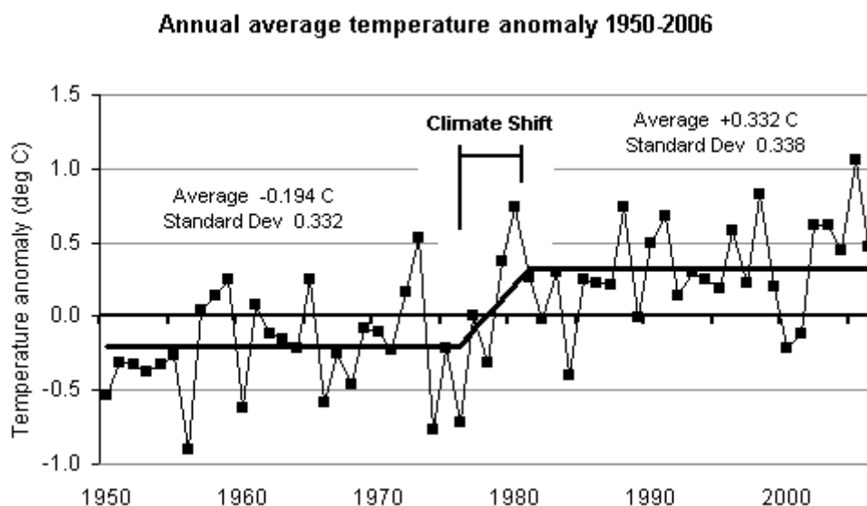
Figure 7-2. An alternative interpretation of Australia's mean temperature record
