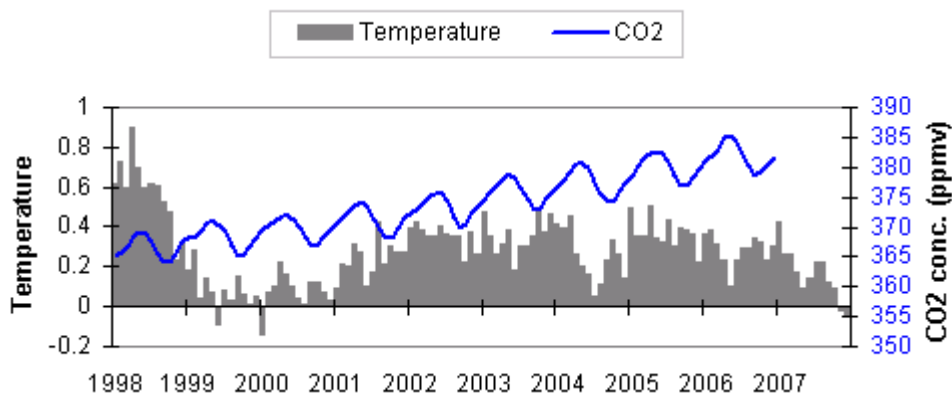
Figure 1-3. Lower tropospheric temperatures according to RSS
