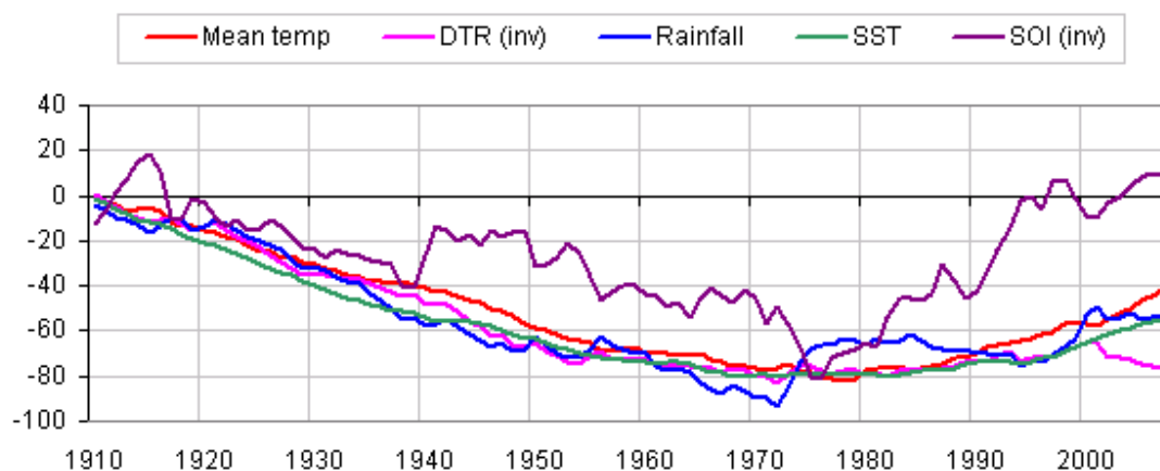
Figure 7-1. Aggregated values of annual averages of key climate factors
