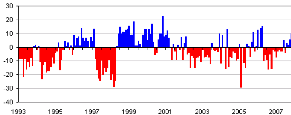
Figure 7-13 Monthly SOI values from January 1993 to December 2007
