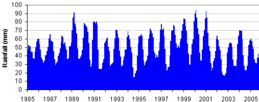
Figure 7-3f. Rainfall across the period of the above graphs
