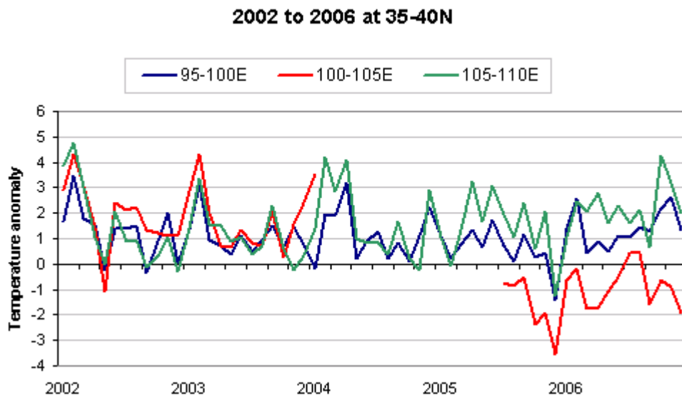
Figure 6-6. HadCRUT3v temperature data from 3 adjacent grid cells
