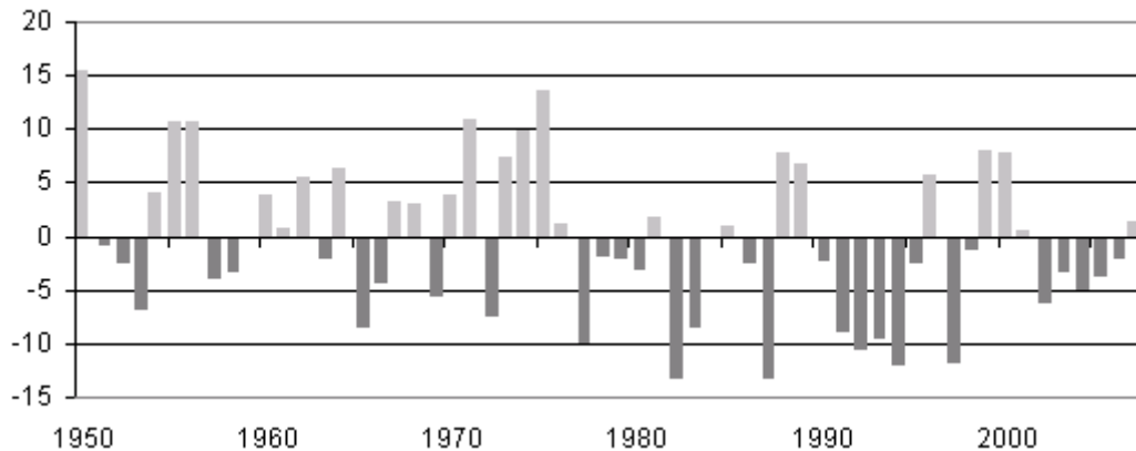
Figure 6-10. Annual average Southern Oscillation Index (1950 - 2006)
