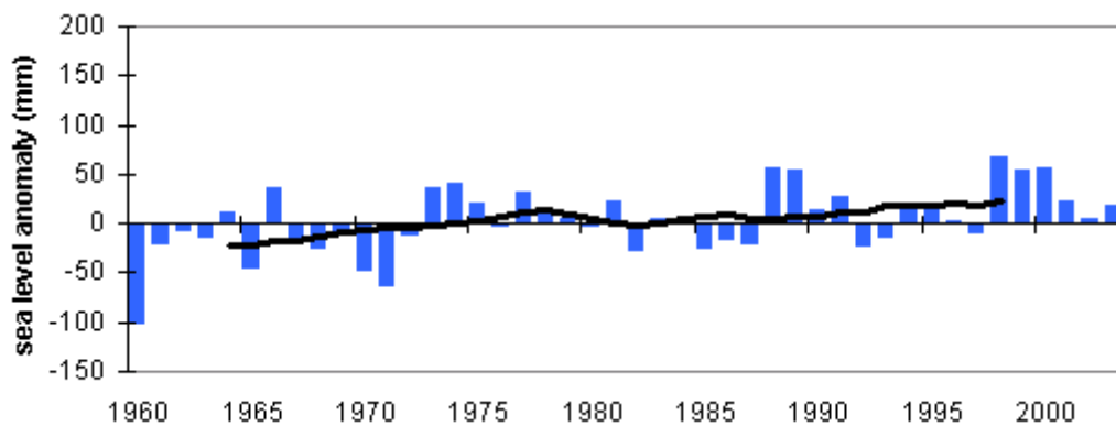
Figure 7-10 Annual average sea level anomaly and 11-year average at Townsville
