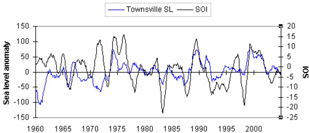
Figure 7-7. Sea level anomalies at Townsville and SOI
