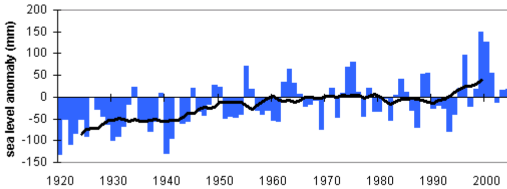
Figure 7-8 Annual average sea level anomaly and 11-year average at Fremantle
