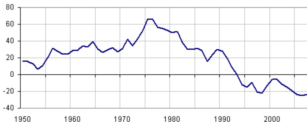
Figure 6-11. Aggregated average annual SOI values
