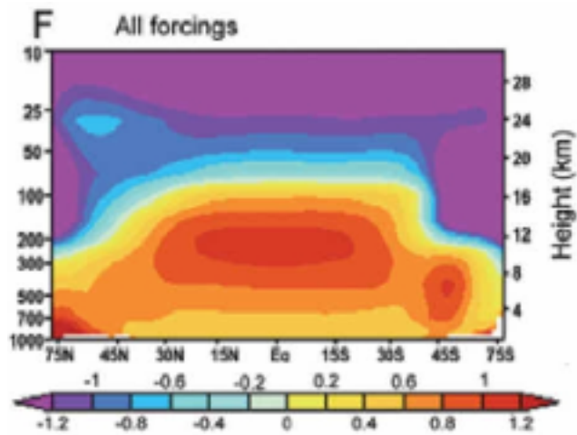
Figure 6-2b. Predicted temperatures trends in the lower troposphere according to the US CCSP (period=1958-1999)
