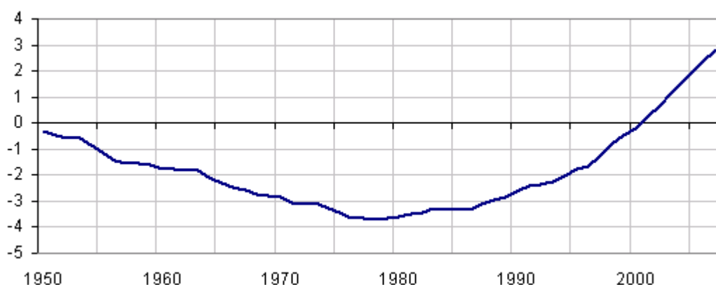
Figure 6-12. Aggregated Global temperature
