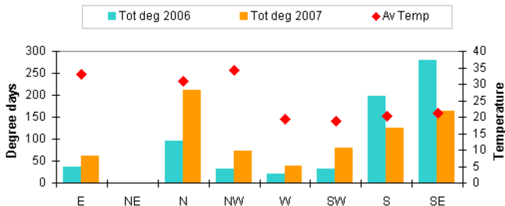
Figure 5-1. Aggregate degrees from each compass point for Laverton (Vic) in December 2006 and 2007.
