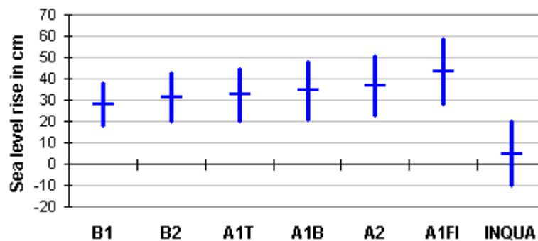
Figure 6-9. Estimated change in sea level by 2099 (range and mid-points). The first 6 from the IPCC and the last from INQUA
