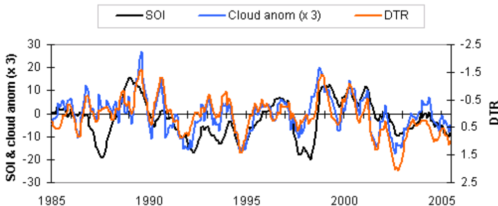
Figure 7-3a. Relationship between SOI, cloud cover and DTR
